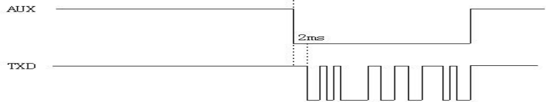
Timing Sequence in Sleep Mode
