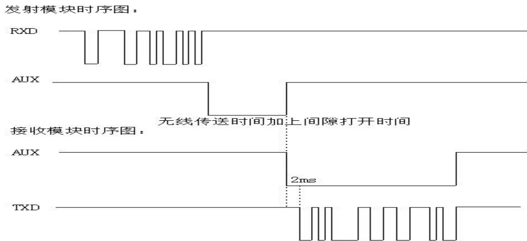
Timing Sequence in Sleep Mode
