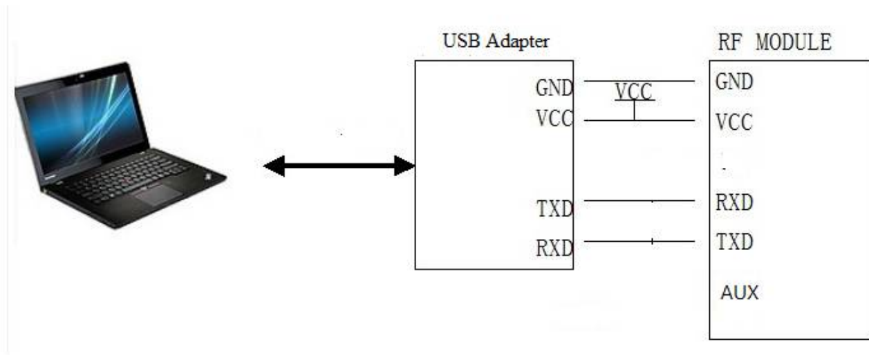
Figure 3: The connection diagram
