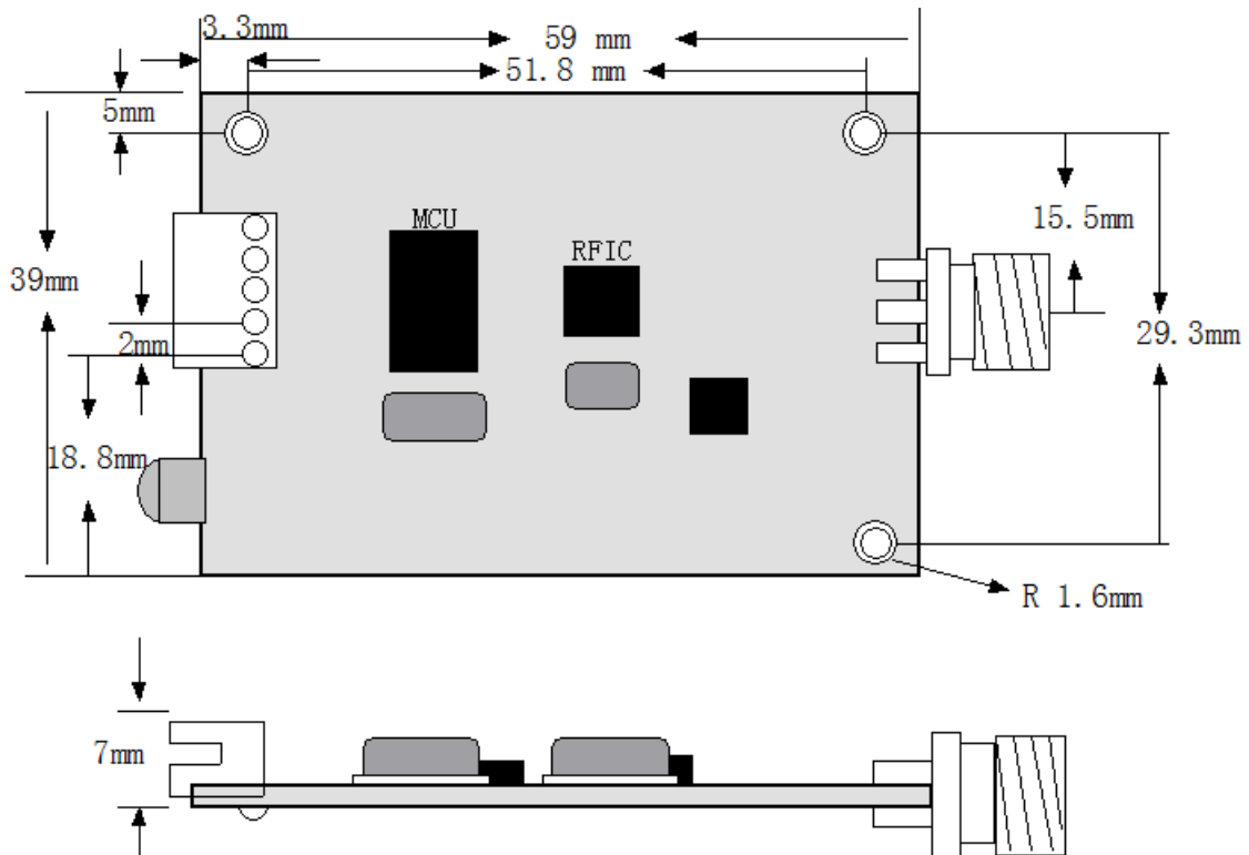
Figure 1: Size of Module
